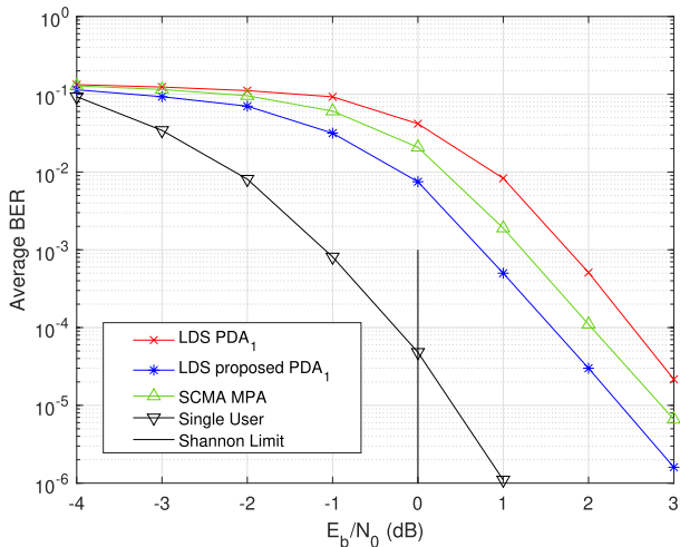
FIGURE 19. QAM with turbo encoding, iteration number = 1, comparisons of C_{4 \times 6} code sets with [32] labeled as LDS.
