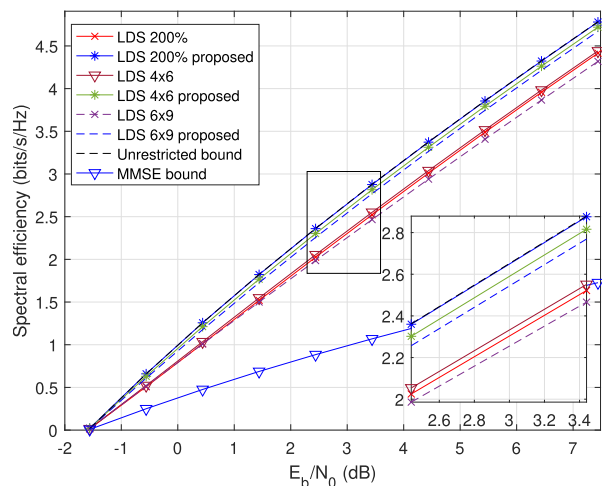
FIGURE 25. Spectral efficiency vs E_b/N_0 of the AWGN channel for BPSK.
