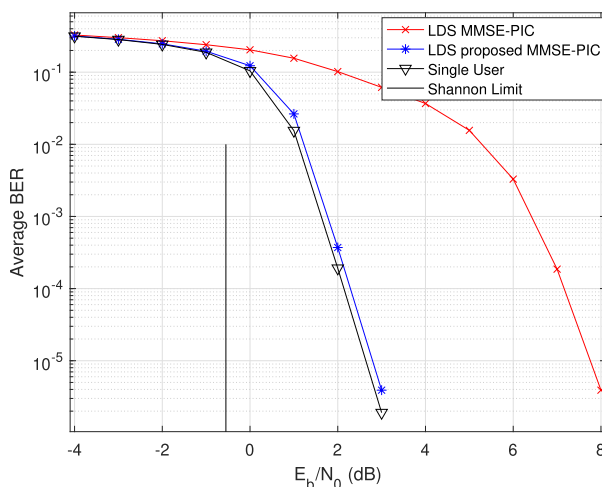
FIGURE 26. Turbo coded BPSK transmission, C_{4 \times 8} code sets with [22] labeled as LDS.
