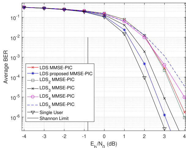
FIGURE 14. BPSK with turbo encoding comparisons of C_{6 \times 9} code sets with [32] labeled as LDS.
