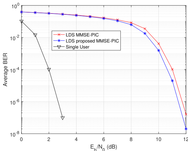
FIGURE 32. Turbo coded BPSK transmission over non-dispersive fading channel, C_{8 \times 16} code sets with [22] labeled as LDS.
