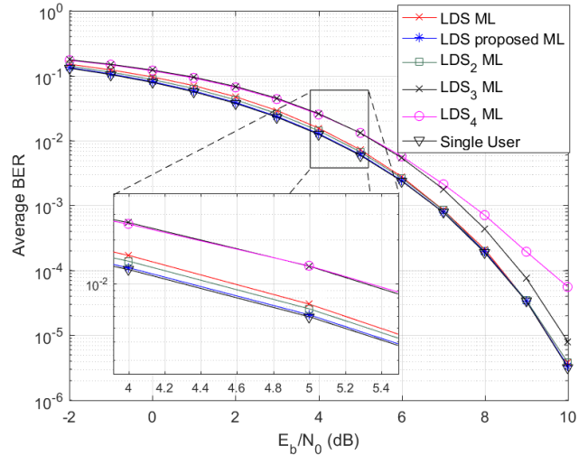
FIGURE 9. Uncoded BPSK case comparisons of \mathbf{C}_{4 \times 6} with labels LDS [32], LDS3 [39], LDS4 [35].
