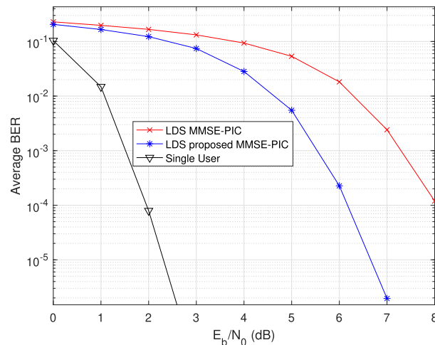
FIGURE 33. Turbo coded BPSK transmission over frequency-selective fading channel, C_{8 \times 16} code sets with [22] labeled as LDS.
