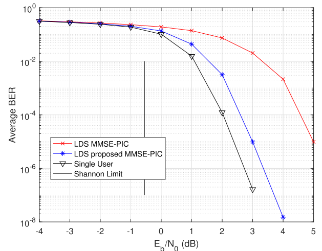
FIGURE 30. Turbo coded BPSK transmission, C_{8 \times 16} code sets with [22] labeled as LDS.
