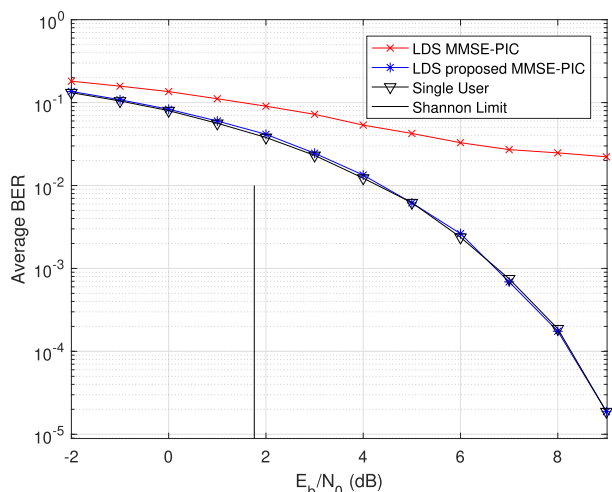
FIGURE 23. Uncoded BPSK transmission, C_{4 \times 8} code sets with [22] labeled as LDS.
