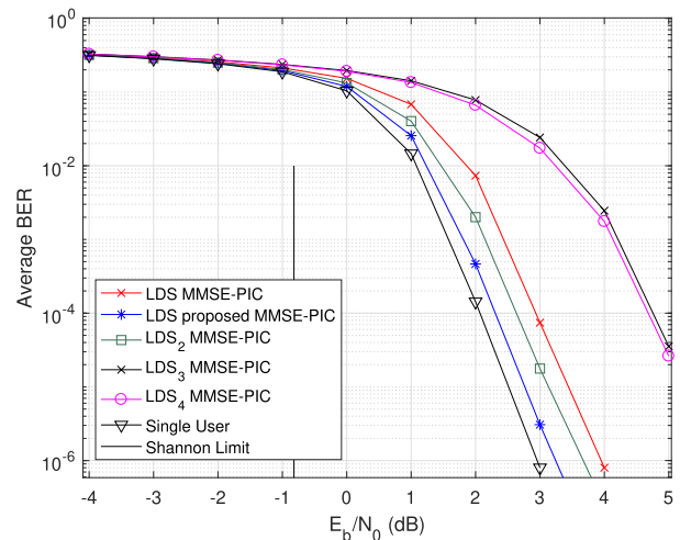
FIGURE 13. BPSK with turbo encoding comparisons of C_{4 \times 6} code sets with labels LDS [32], LDS3 [39], LDS4 [35].
