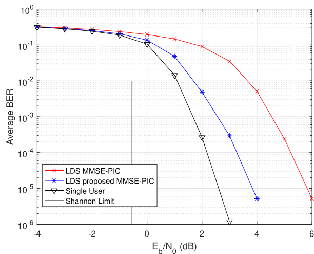
FIGURE 28. Turbo coded BPSK transmission, C_{6 \times 12} code sets with [22] labeled as LDS.
