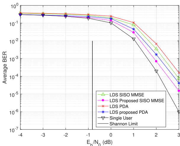
FIGURE 15. BPSK with turbo encoding comparisons of C_{4 \times 6} code sets with [32] labeled as LDS.
