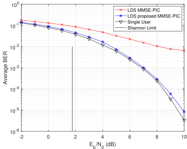
FIGURE 27. Uncoded BPSK transmission, C_{6 \times 12} code sets with [22] labeled as LDS.
