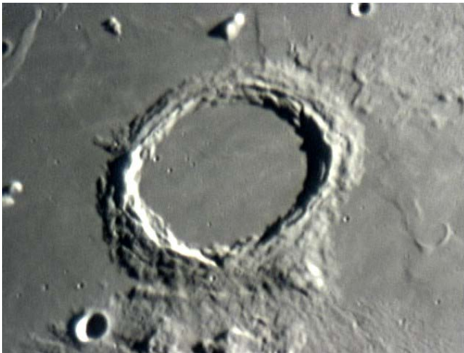
Archimedes crater
