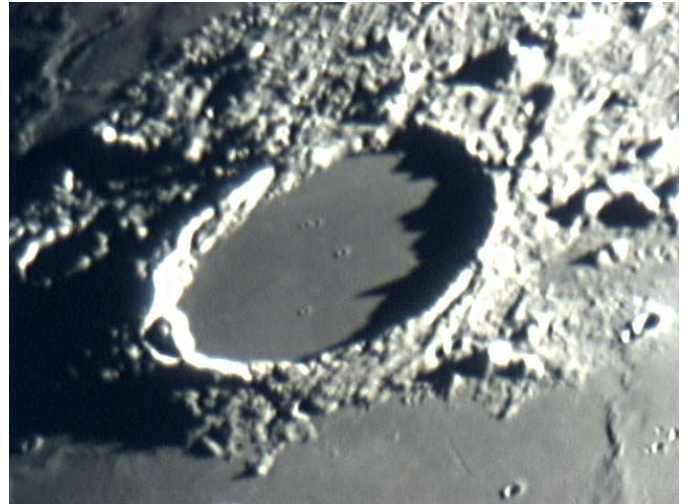
Plato crater
