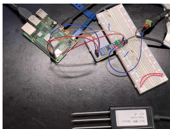
Fig. 6: Raspberry Pi to MAX485 to Soil Sensor.
