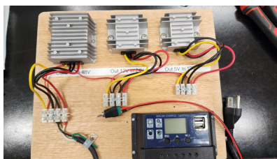
Fig. 10: Power Bank Bus Converters.
