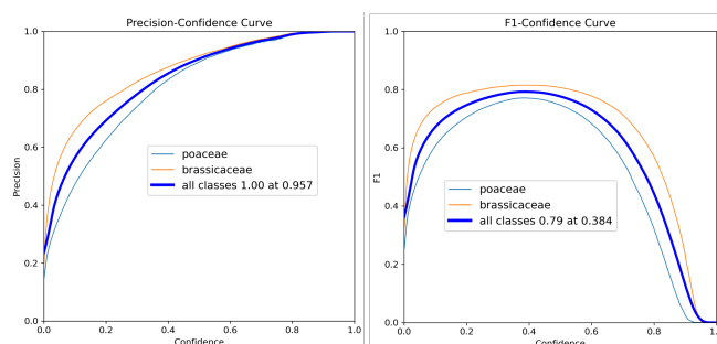
Fig. 12: Precision Confidence and F1 Confidence Curves.
