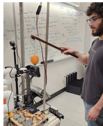
Fig. 4: Fruit Picking with the Robotic Arm.
