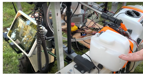
Fig. 3: Spot Sprayer (Iron-ton ATV).
