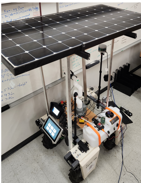
Fig. 11: SunPower Mounted on SARDOG.
