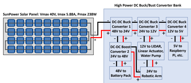
Fig. 9: Energy Harvesting System.
