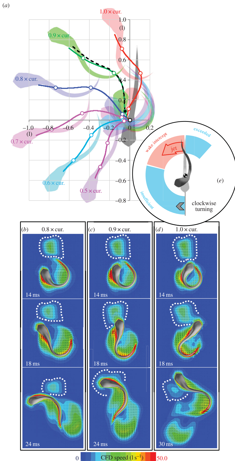
Figure 10. Simulated C-starts for a fish larva in the inertial flow regime ( Re 6000), based on the body kinematics observed in [15], to explore the effects of Re on wake interception. (a) Predicted trajectories for a range of maximum body curvatures. (Black dashed trajectory = trajectory-effect model, starting from the solid black dot position at 14 ms). (b–d) Flow velocity field for simulations at 0.8, 0.9 and 1.0 times the originally observed body curvature. (e) Summary of the wake-interception effect in larval fish. Fish larvae will intercept their wake during a C-start if their turning angle is between 100^\circ and 180^\circ ; fish larvae are able to undershoot but not overshoot their wake, possibly due to Re effects.
